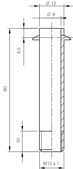
Nippel EN30 Ø 12 mm L 60 mm M12x1 Nipple EN30 Ø 12 mm L 60 mm M12x1
