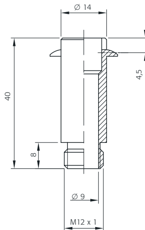
Nippel EN32 Ø 14 mm M12x1 Nipple EN32 Ø 14 mm M12x1
