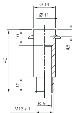
Nippel EN32 Ø 14 mm L 40 mm M12x1 Nipple EN32 Ø 14 mm L 40 mm M12x1
