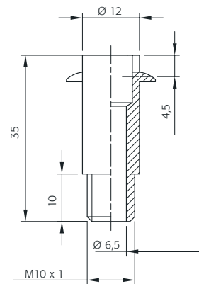
Nippel Ø 12 mm L 35 mm M10x1 Nipple Ø 12 mm L 35 mm M10x1
