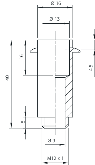
Nippel Ø 16 mm L 40 mm M12x1 Nipple Ø 16 mm L 40 mm M12x1
