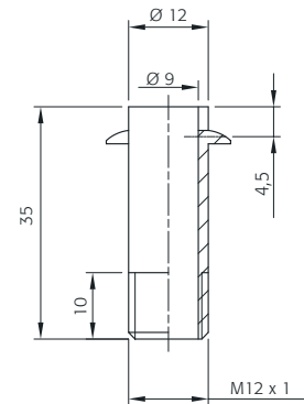
Nippel N20/21S Ø 12 mm L 35 mm M12x1 Nipple N20/21S Ø 12 mm L 35 mm M12x1
