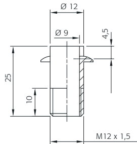
Nippel N16 Ø 12 mm L 25 mm M12x1,5 Nipple N16 Ø 12 mm L 25 mm M12x1,5
