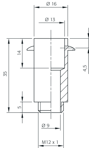
Nippel Ø 16 mm L 35 mm M12x1 Nipple Ø 16 mm L 35 mm M12x1
